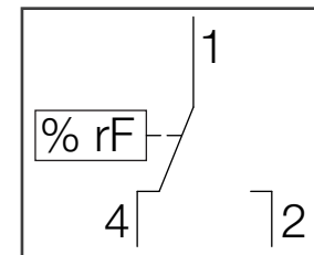
Abbildung 2: Anschluss HYG12 / Figure 2: Connection of HYG12
