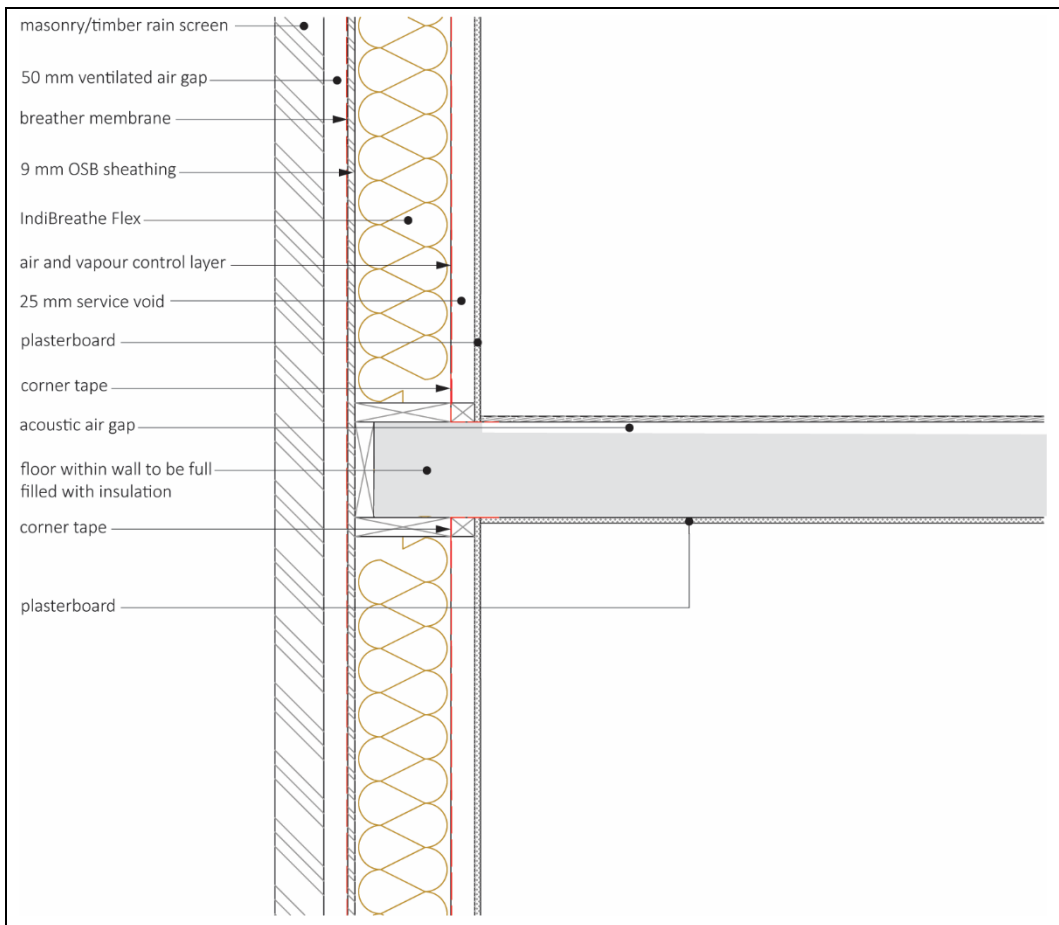
Figure 3 Wall to intermediate floor junction detail
