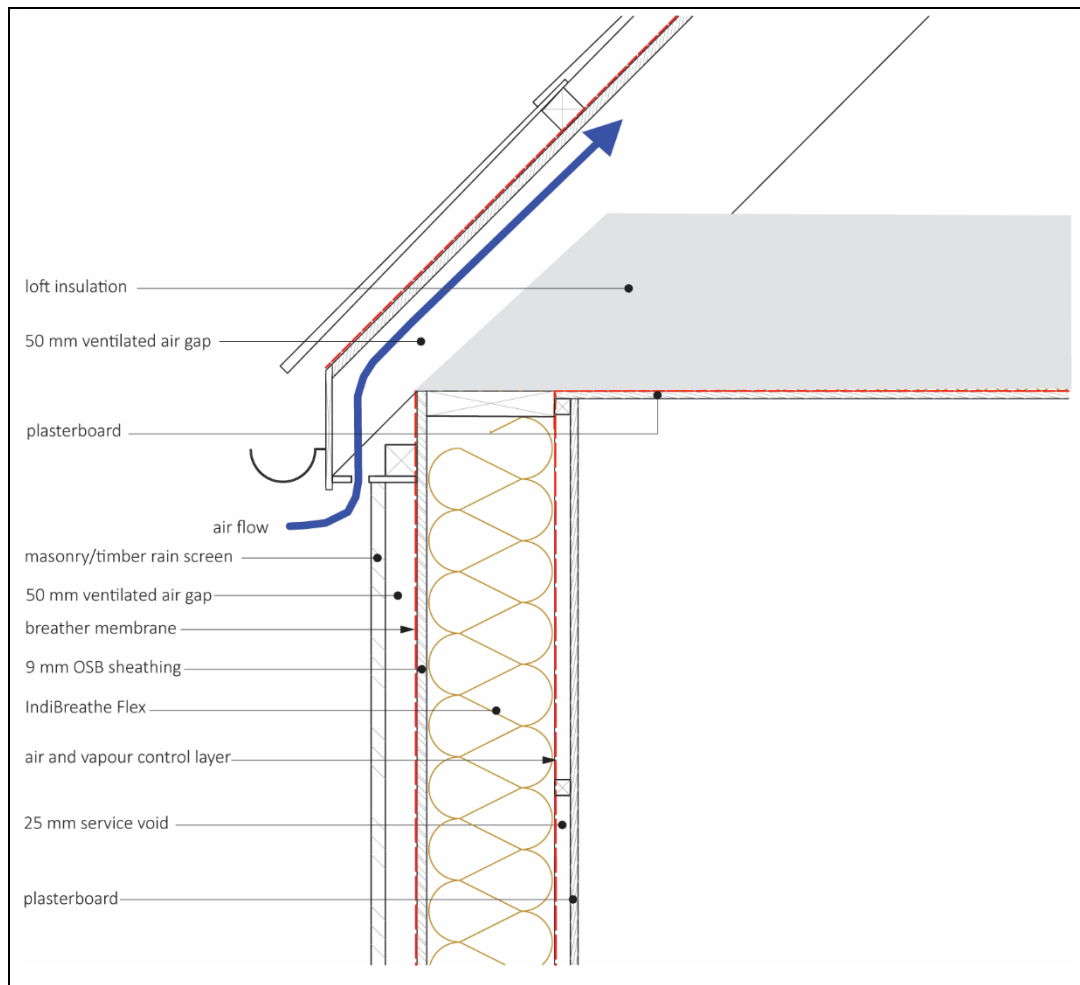
Figure 5 Wall to roof junction detail
