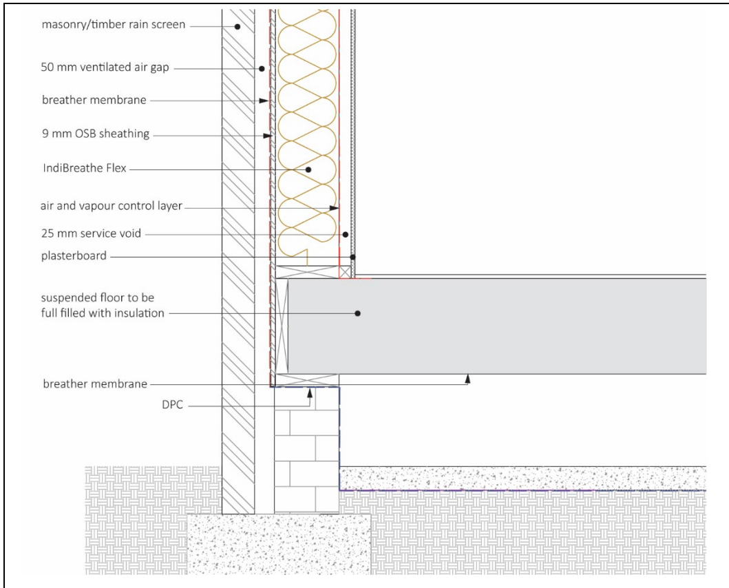
Figure 2 Wall to suspended floor junction detail
