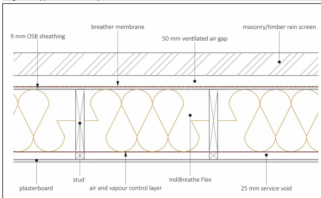
Figure 1 Typical wall build up detail
